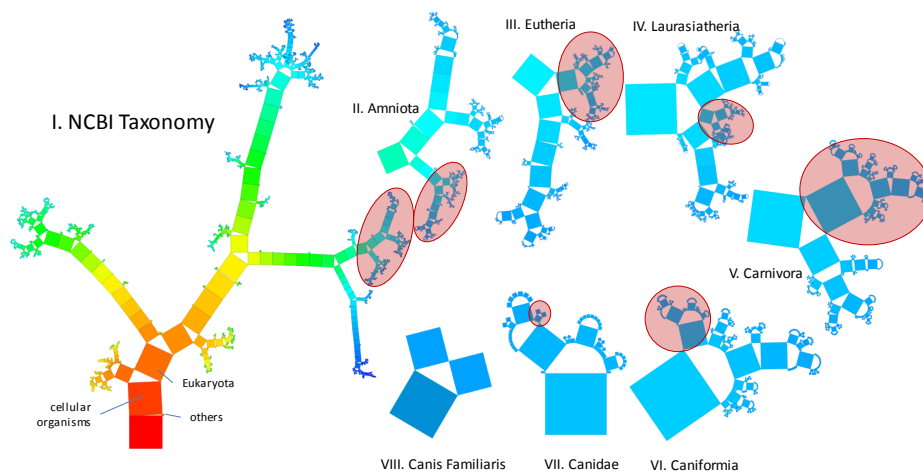
Fig. 10. NCBI taxonomy hierarchically classifying species; rectangles sizes indicate the number of species in a subtree, color encodes the depth; an example for exploring the taxonomy by semantic zooming is provided.
