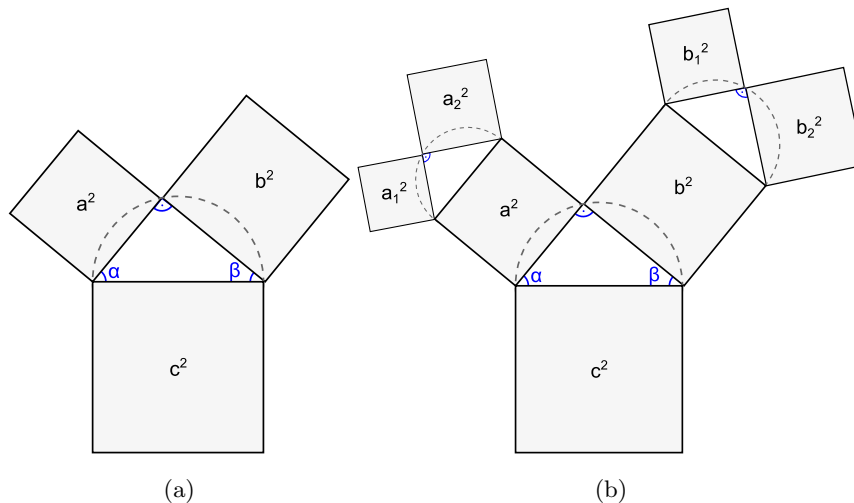
Fig. 2. Illustration of the traditional Pythagoras Tree approach: (a) a single binary branch; (b) recursively applied branching step.
