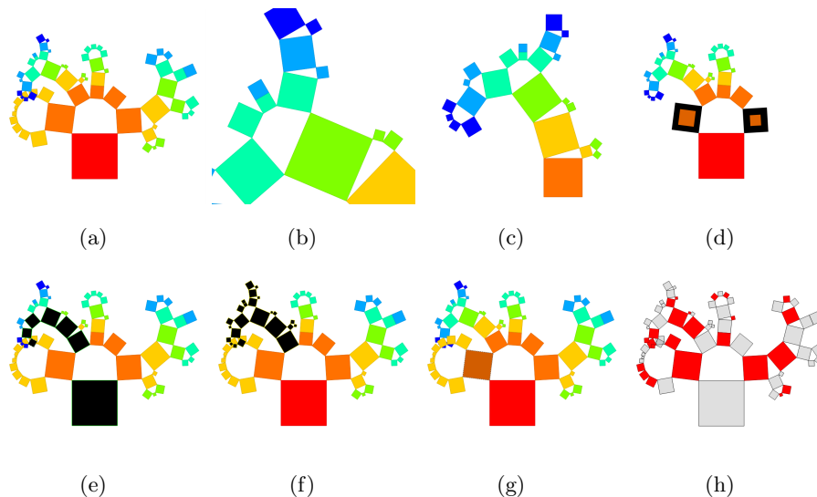
Fig. 8. Interaction in Generalized Pythagoras Trees: (a) sample hierarchy in default representation, (b) geometric zooming, (c) selected subhierarchy, (d) collapsed nodes, (e) highlighted path, (f) highlighted subhierarchy, (g) subhierarchy moved to front, and (h) highlighting by search.
