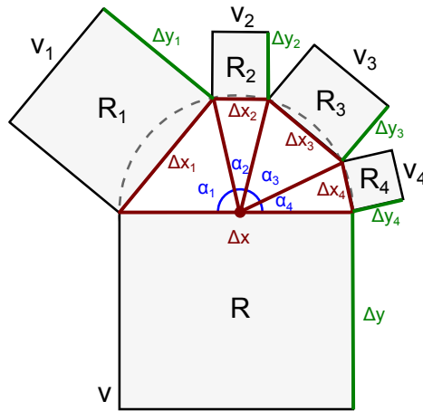
Fig. 4. Polygonal split of Generalized Pythagoras Trees creating an n -ary branch.
